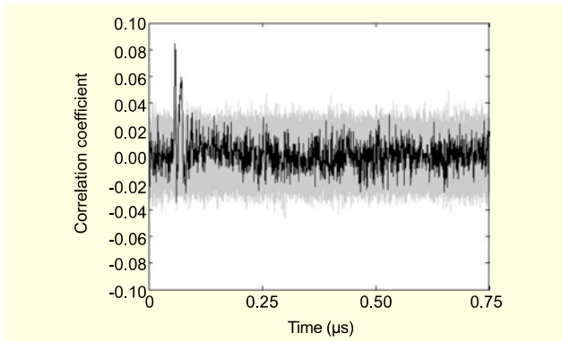
Fig. 17. Second-order DEMA traces of all 256 key hypotheses.
