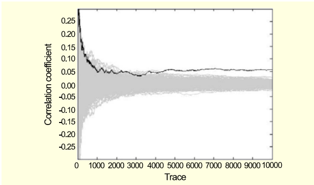
Fig. 16. Second-order DPA: correlation coefficient for various numbers of traces.
