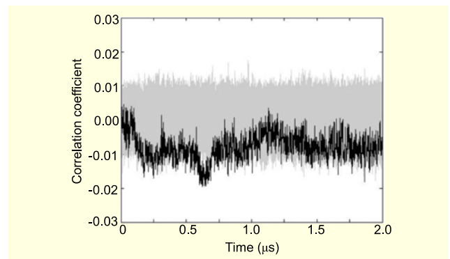
Fig. 20. Result of the second-order DPA attack using the preprocessing function pre(P) = |P - E(P)| .
