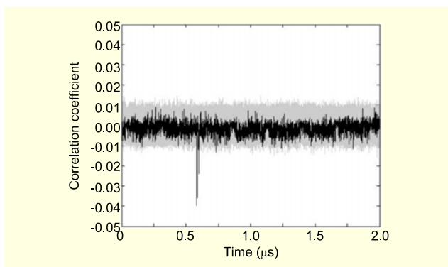
Fig. 21. Result of the second-order DEMA attack using the preprocessing function pre(P) = |P - E(P)| .
