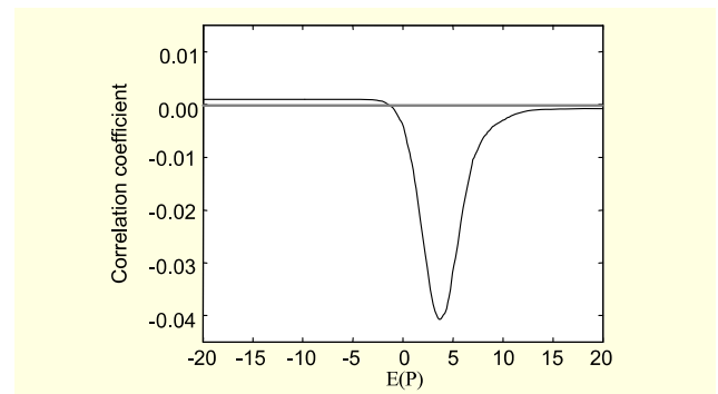
Fig. 19. Correlation coefficient for different offsets of the mean E(P) in case of the EM traces.
